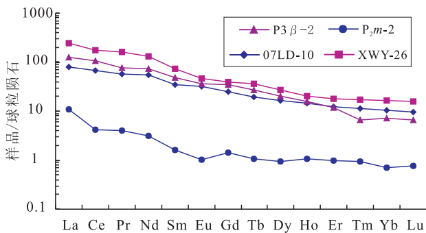
07LD-10-罗甸晚二叠世辉绿岩; XWY-26-贵州西部玄武岩; P 3 β-2-晴隆大厂玄武岩 07LD-10-Late Permian Diabase in Luodian; XWY-26-Basalt in west of Guizhou; P 3 β-2-Basalt in Dachang of Qinglong 图7 区域基性-超基性岩及水银洞矿区茅口组灰岩稀土元素球粒陨石标准化模式图
