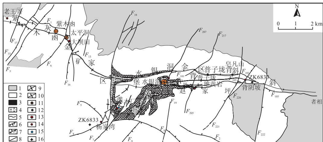
1-永宁镇组;2-夜郎组;3-长兴+大隆组;4-龙潭组;5-地层界线;6-正断层;7-逆断层;8-性质不明断层;9-背斜轴;10-向斜轴;11-金矿床;12-金矿点;13-汞矿床;14-汞矿点;15-铊矿点;16-钻孔及采样位置 1-Yonglinzhen formation; 2-Yelang formation; 3-Changxing and Dalong formation; 4-Longtan formation; 5-the stratum borderline; 6-measured and inferred normal fault and its number; 7-measured and inferred reverse fault and its number; 8-undefined fault; 9-axis of anticline; 10-axis of syncline; 11-gold deposit; 12-gold occurrence; 13-mercury deposit; 14-mercury occurrence; 15-thallium occurrence; 16-location of drill and sampling
