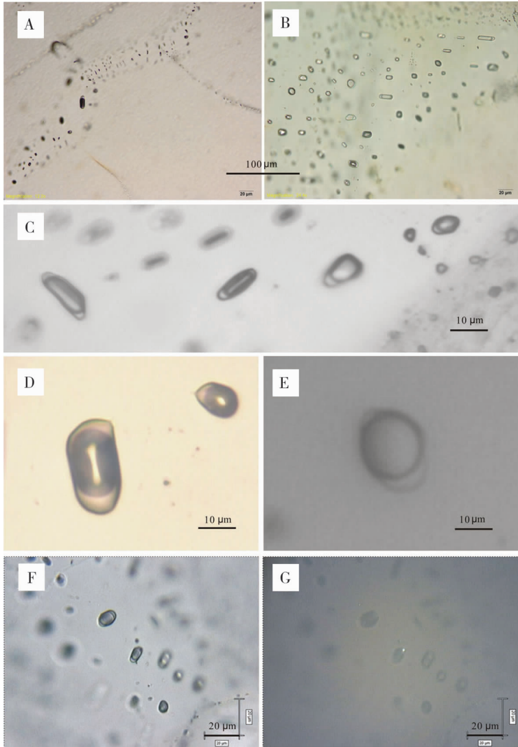
A-合成包裹体沿裂隙分布(实验编号 3 # );B,C-气液两相包裹体,气相所占比例较大,气液比均一(实验编号 2 # 、3 # );D,E-低密度气液相包裹体,气相所占比例约 70%(实验编号 2 # );F,G-包裹体边缘含不透明子矿物,反射光下反光强烈,估计是 Ag 或 Ag 的氯化物(实验编号 3 # ) A-Synthetic fluid inclusions distributed along dendritic cracks of quartz crystals (experimental number 3 # ); B,C-Liquid-Vapor type fluid inclusions with a large and uniform proportion of gas (experimental number 2 # , 3 # ); D,E-Low density liquid-vapor type fluid inclusions with approximately 70% of gas (experimental number 2 # ); F,G-Fluid inclusions contain one or more opaque particles, hypothesized to be Ag or AgCl based on their color when viewed under reflected light (experimental number 3 # )
