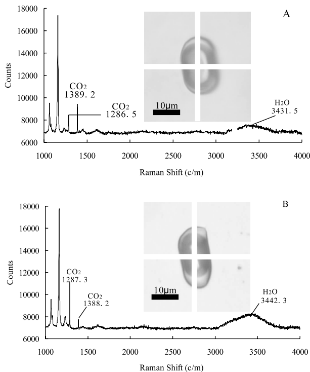
图 4 NaCl-H 2 O-CO 2 体系合成包裹体激光喇曼图谱 Fig. 4 Laser Raman spectra of synthetic fluid inclusions in the NaCl-H 2 O-CO 2 system
